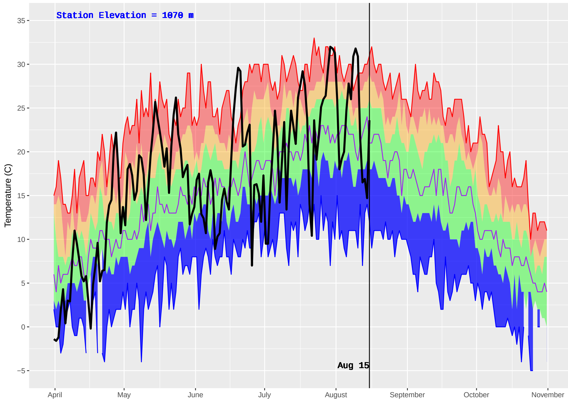
MEADOW LAKE (236) : Historical (1991–2016) and Current (2018) Daily Temperature
