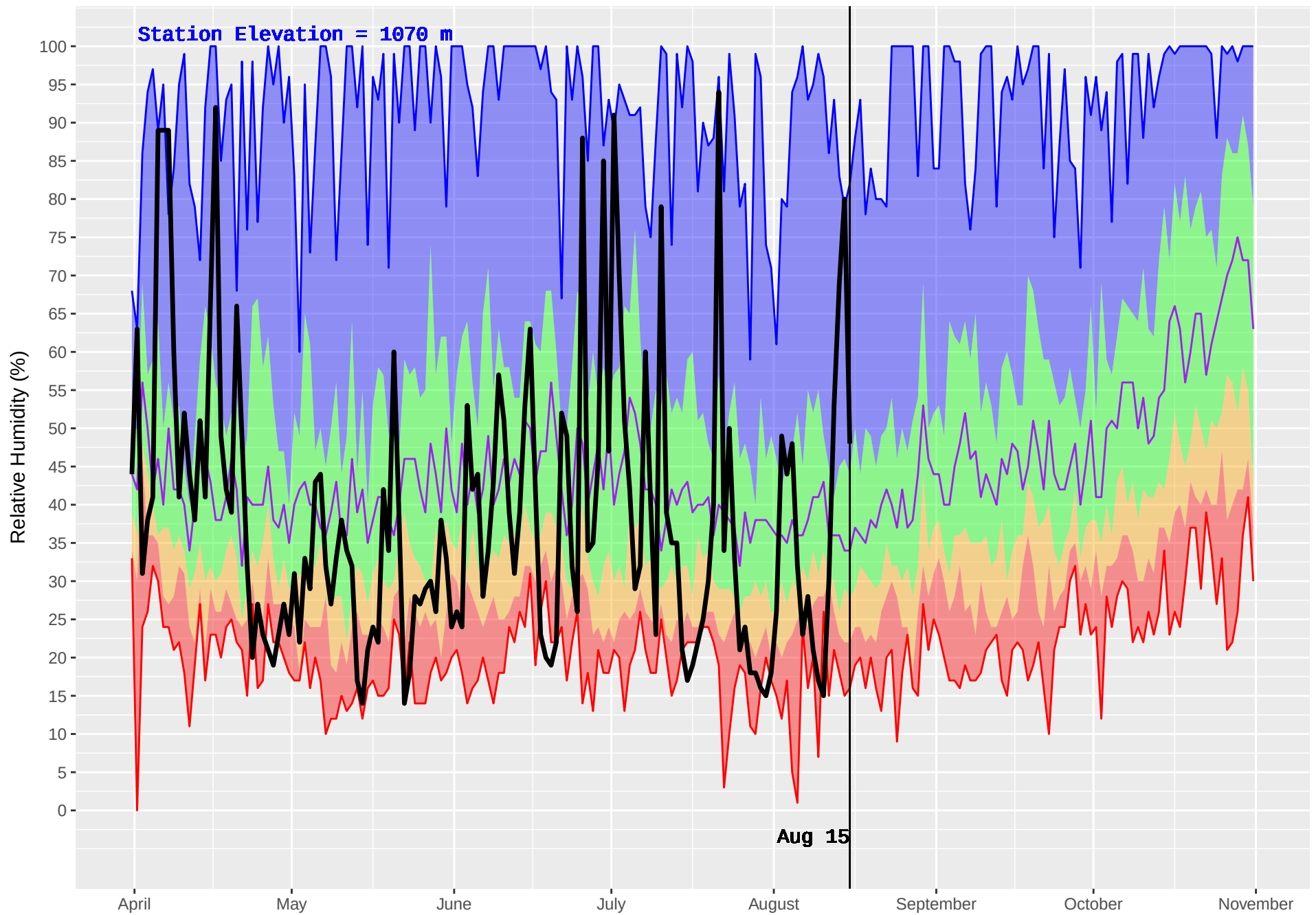
MEADOW LAKE (236) : Historical (1991–2016) and Current (2018) Daily Relative Humidity
