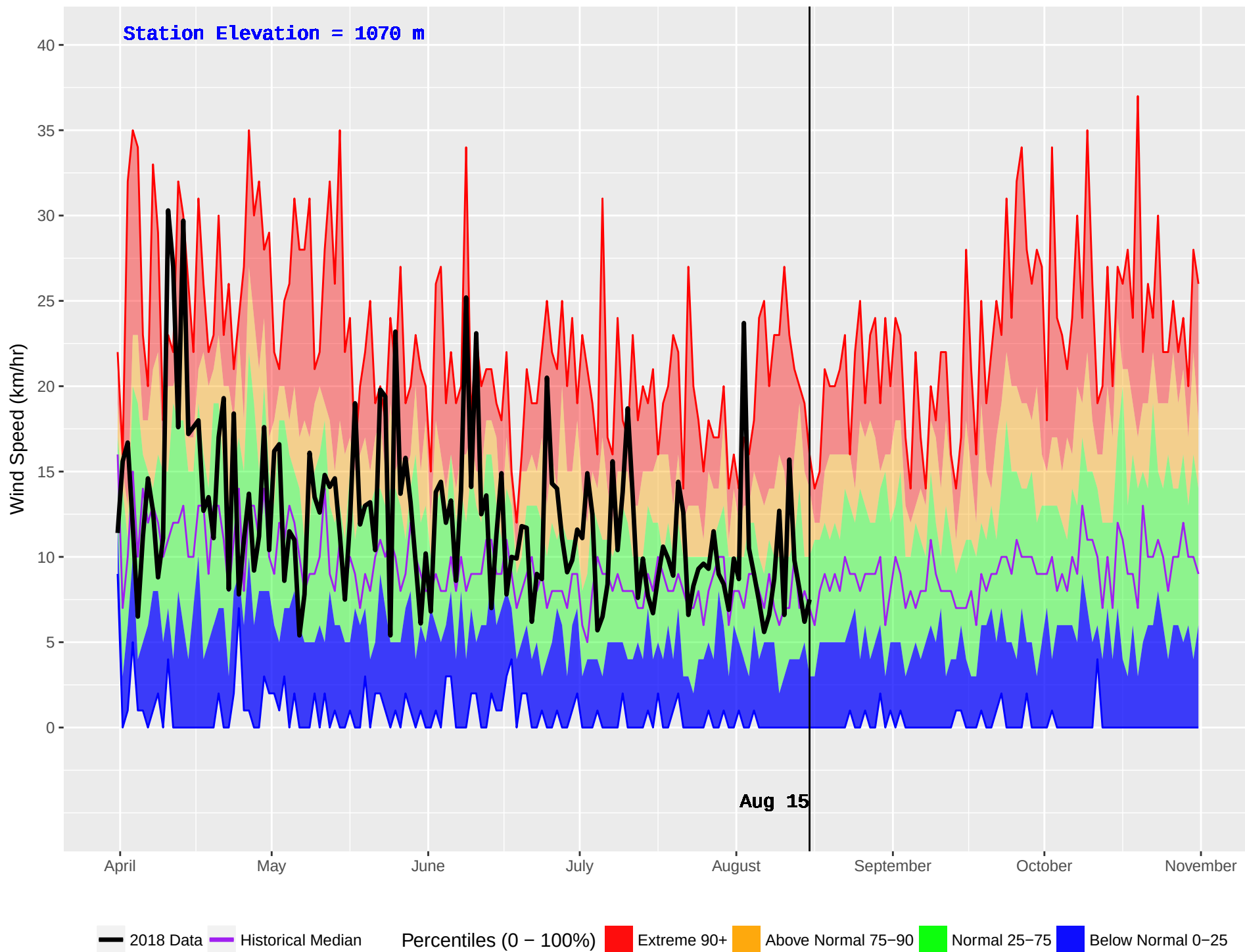
MEADOW LAKE (236) : Historical (1991–2016) and Current (2018) Daily Wind Speed
